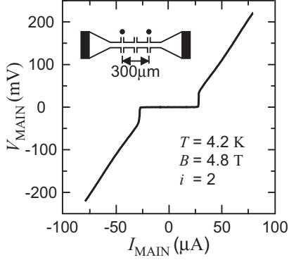
FIG. 2: I - V characteristics of the main channel.
